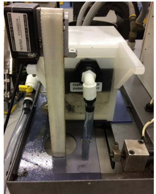
Oil collecting in Keller Skimallessor Tank.
