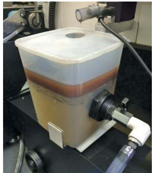
Oil collecting in Keller Skimallessor Tank.
